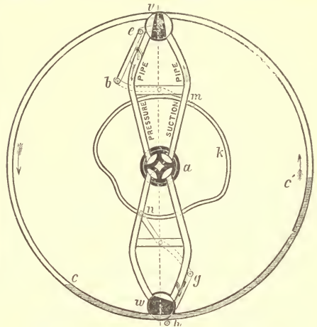
FIG. 7.—Doyle and Martin's Rotary Air Pump.
